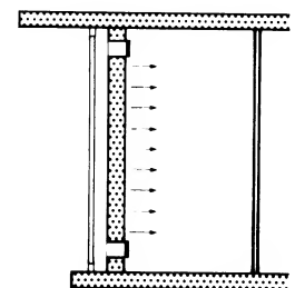
⑫ Winter night: thoroughly warmed wall acts as a radiant heat surface in the room; with the upper and lower flaps closed, the stationary layer of air between the external glazing and the Trombè wall helps to reduce the heat loss
